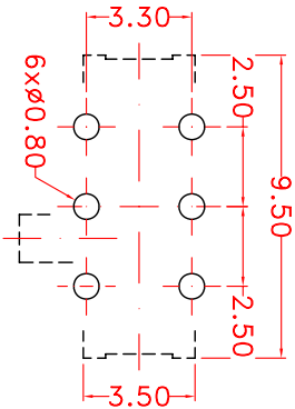
PIERCING PLAN
