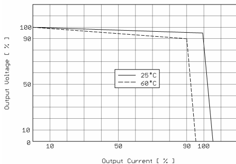
TYP. CURRENT LIMITED CURVE
